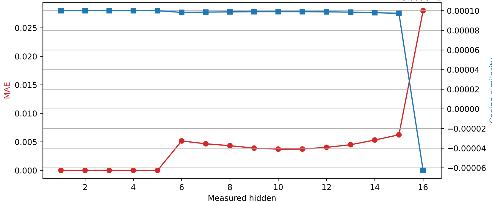
Llama-3.2-1B | Quantized layer 5 | float64 → int8
