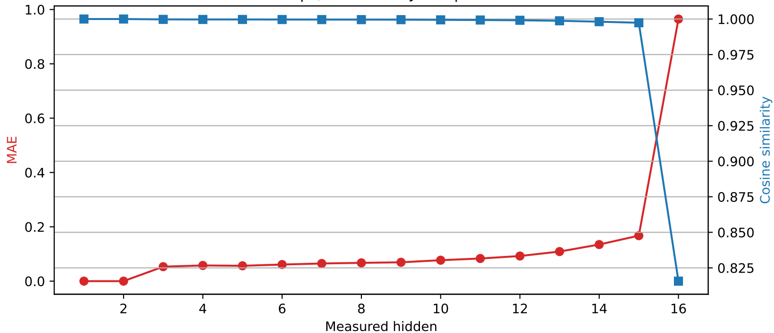
Llama-3.2-1B | Quantized layer 2 | float32 → int4
