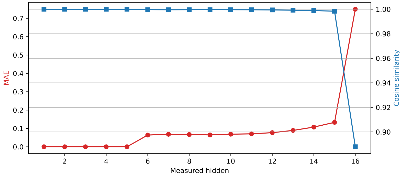
Llama-3.2-1B | Quantized layer 5 | float32 → int4
