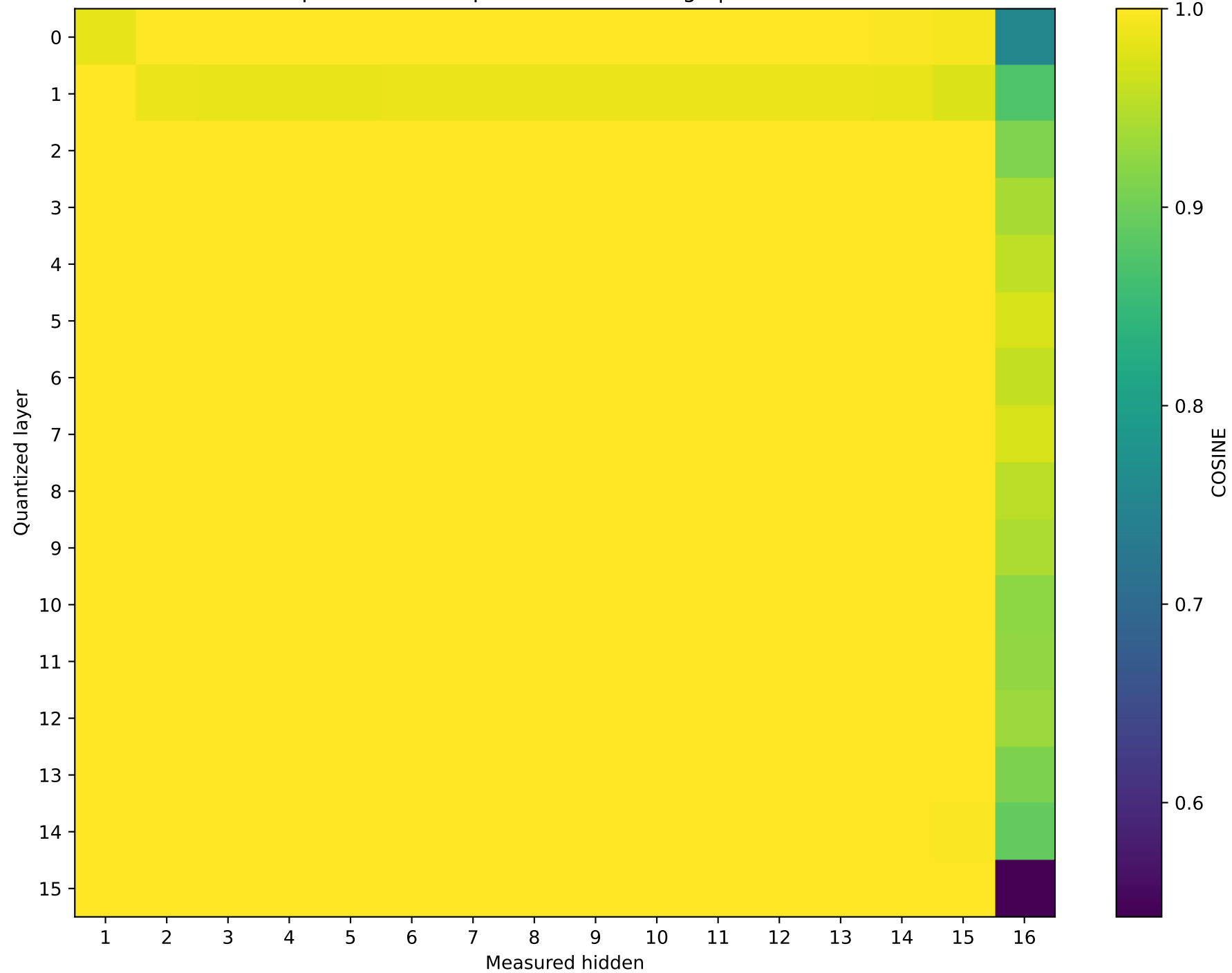
Llama-3.2-1B Prompt 0: cos sim representation damage | float64 → int4
