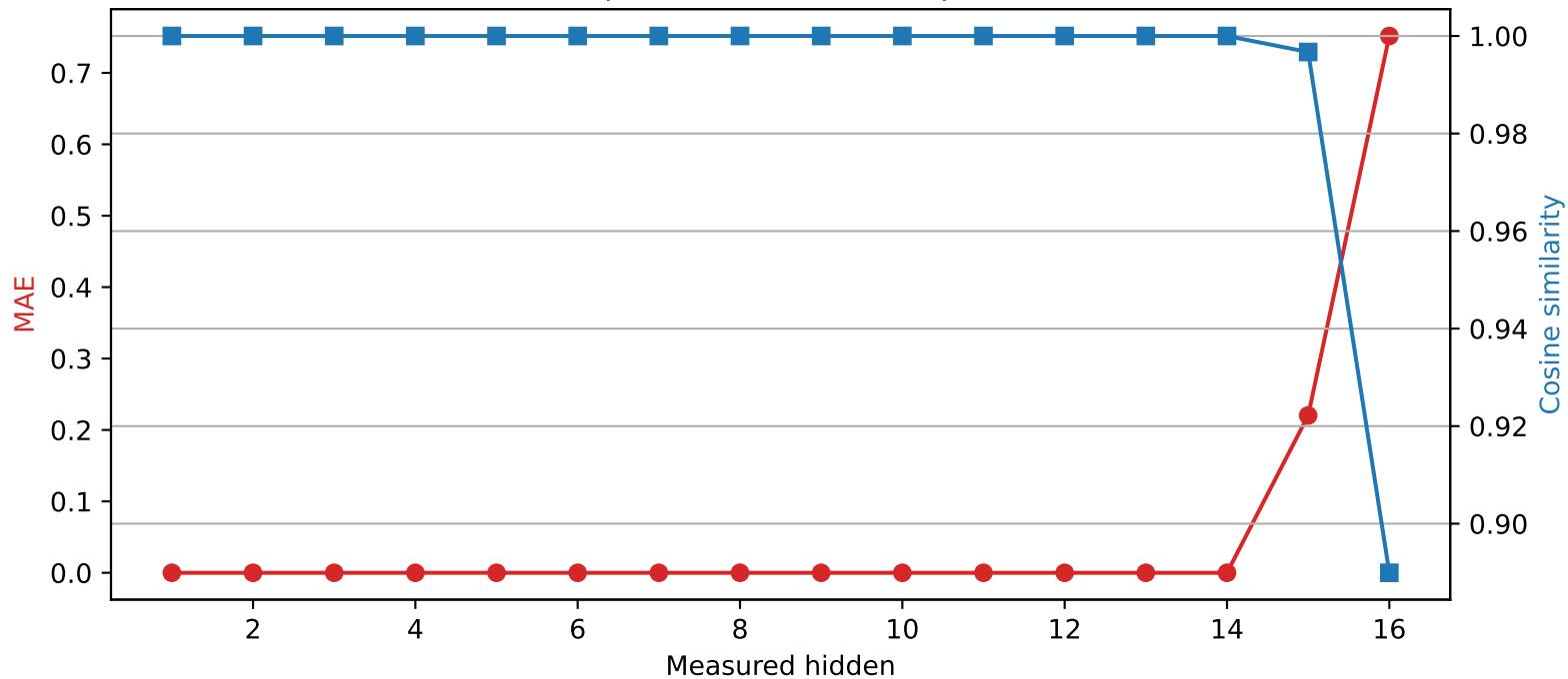
Llama-3.2-1B | Quantized layer 14 | float64 → int4
