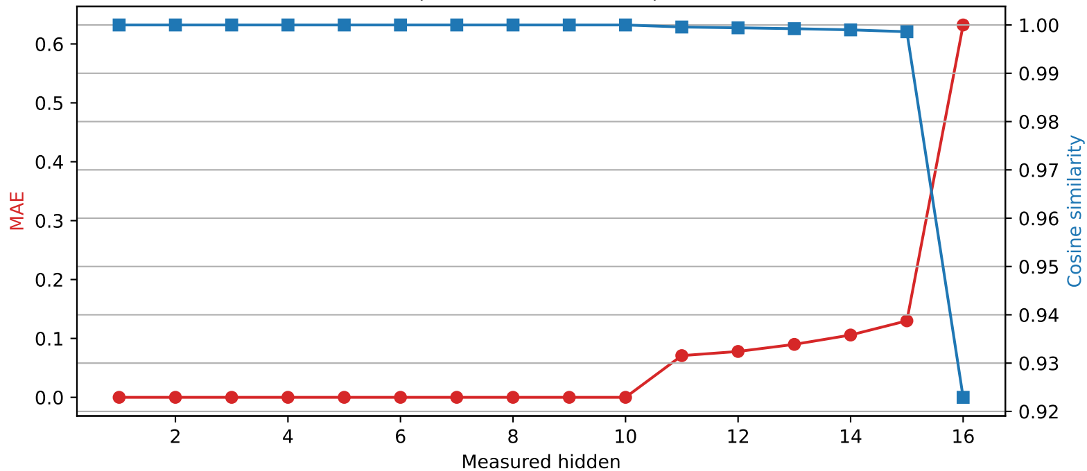
Llama-3.2-1B | Quantized layer 10 | float64 → int4
