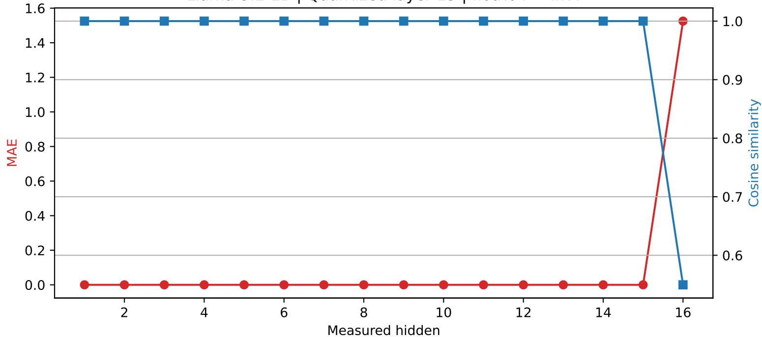
Llama-3.2-1B | Quantized layer 15 | float64 → int4
