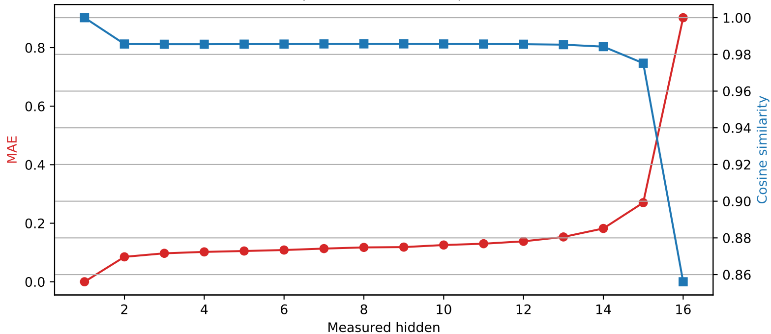
Llama-3.2-1B | Quantized layer 1 | float64 → int4
