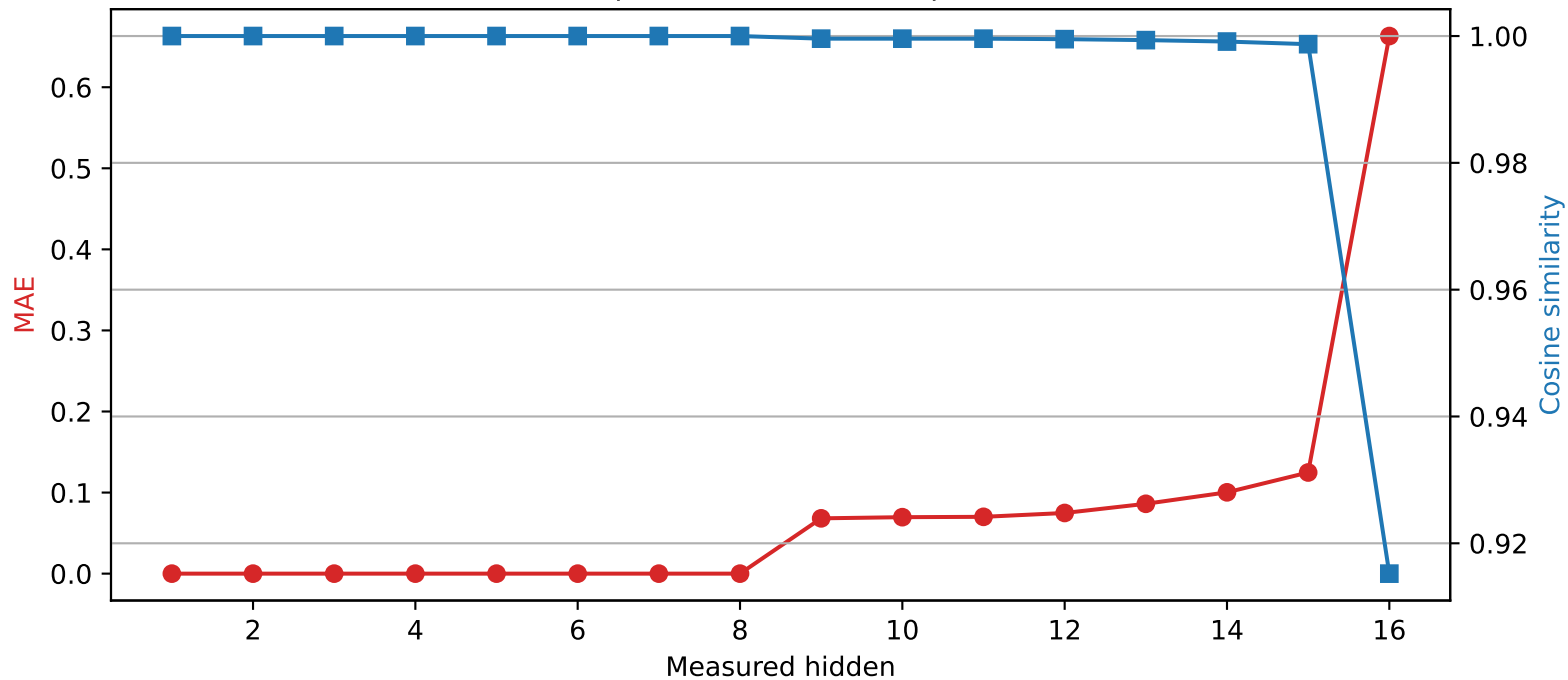
Llama-3.2-1B | Quantized layer 8 | float64 → int4
