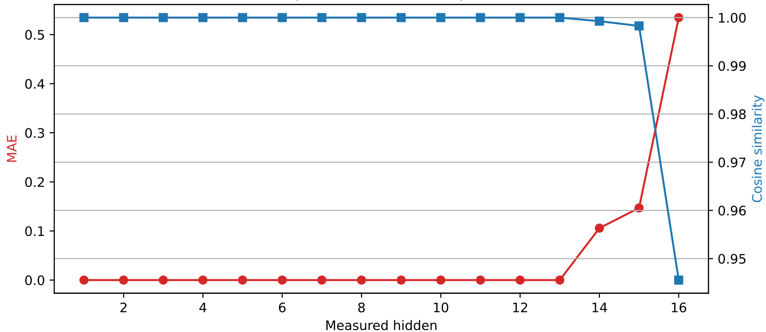
Llama-3.2-1B | Quantized layer 13 | float64 → int4
