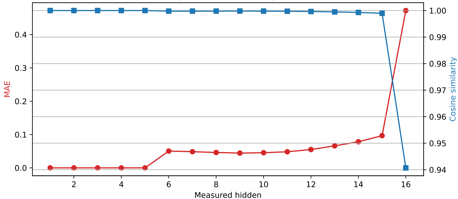
Llama-3.2-1B | Quantized layer 5 | float32 → int2
