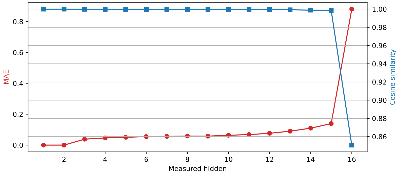
Llama-3.2-1B | Quantized layer 2 | float32 → int2
