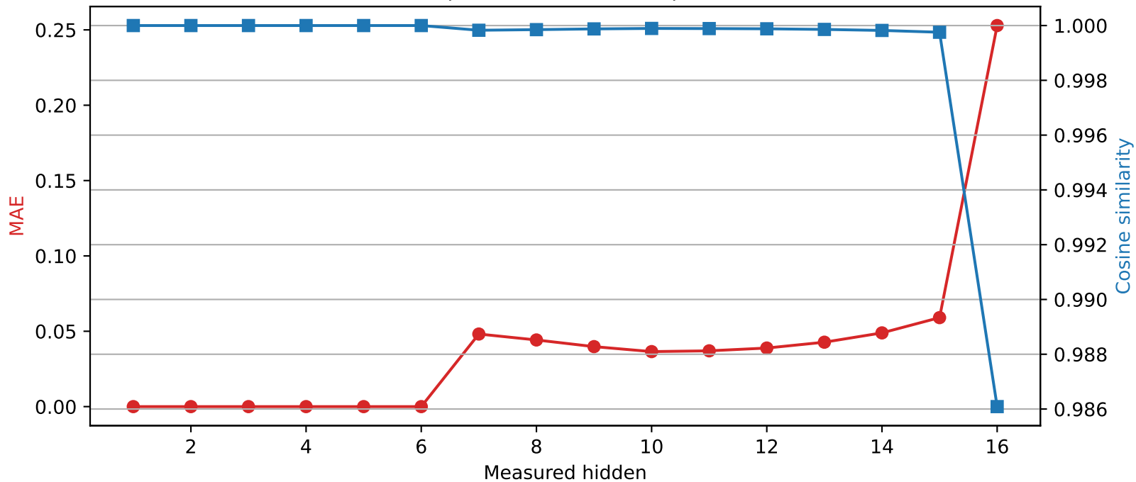
Llama-3.2-1B | Quantized layer 6 | float32 → int2
