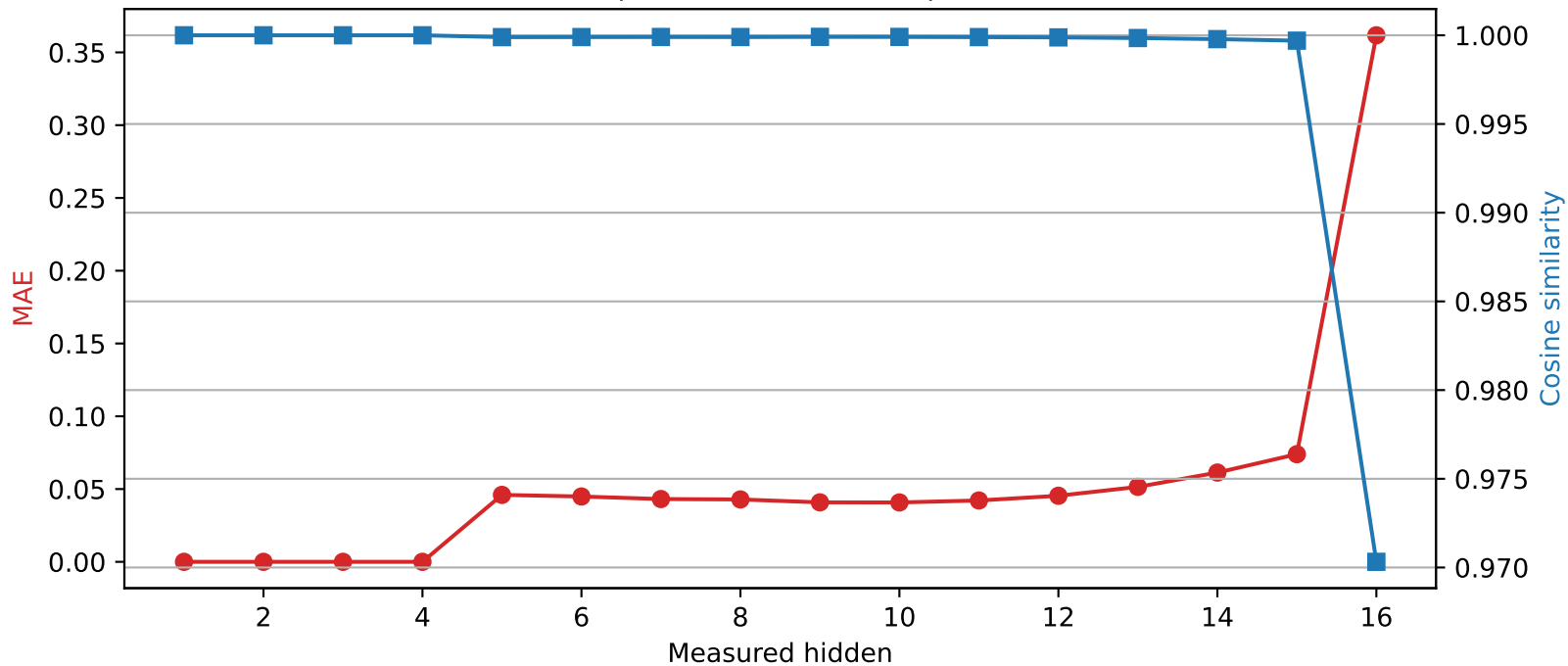
Llama-3.2-1B | Quantized layer 4 | float64 → int2
