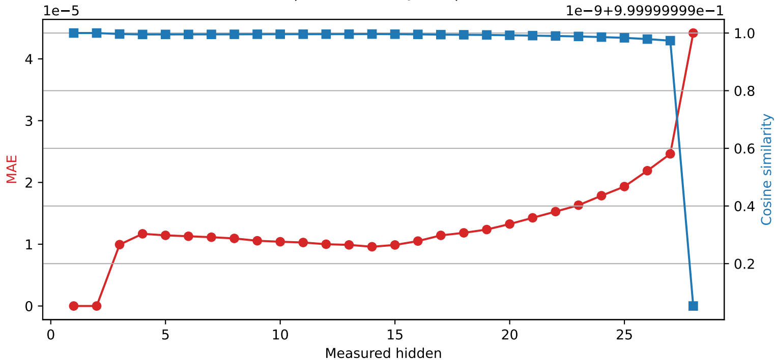
Llama-3.2-3B | Quantized layer 2 | float32 → int16
