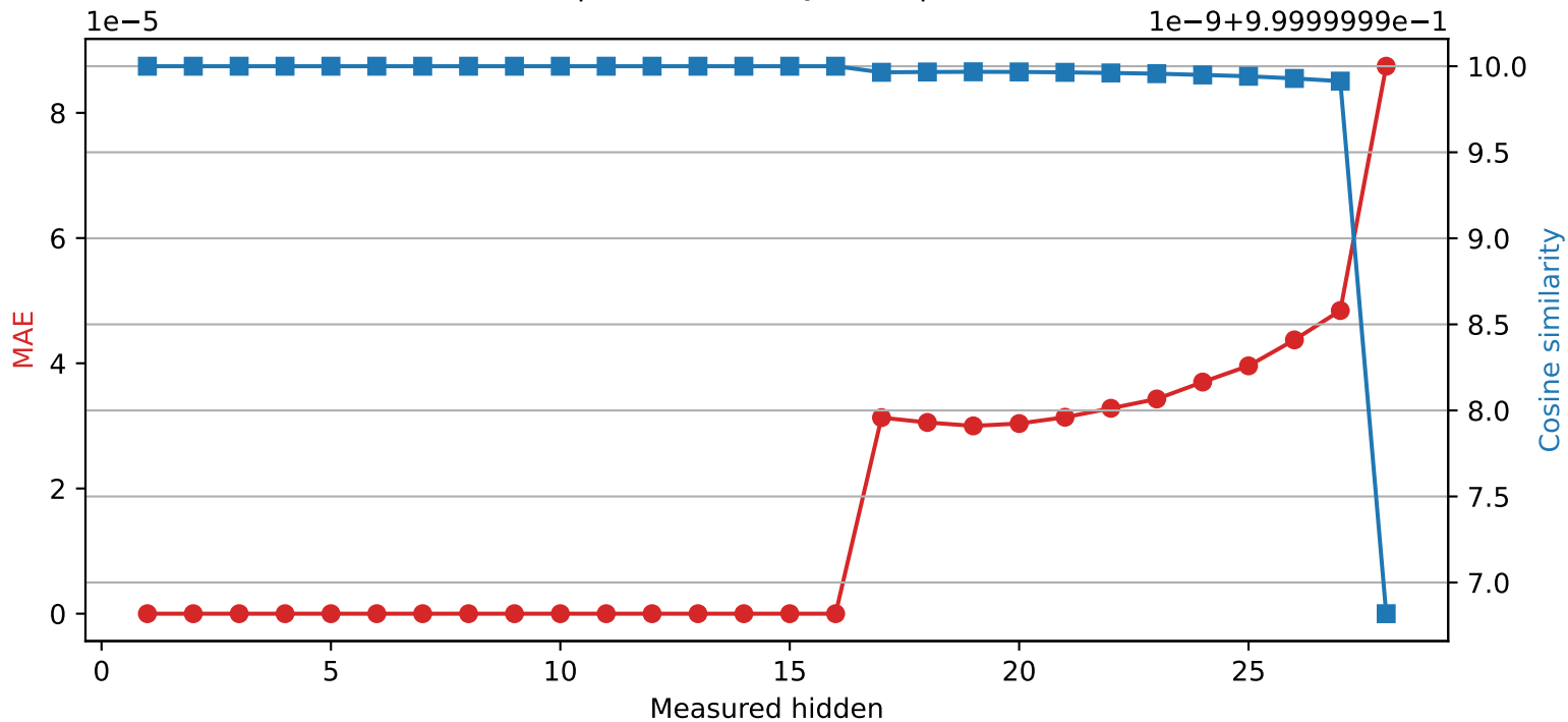
Llama-3.2-3B | Quantized layer 16 | float32 → int16
