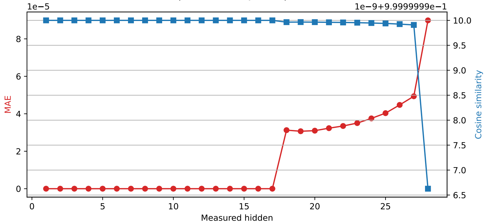
Llama-3.2-3B | Quantized layer 17 | float32 → int16
