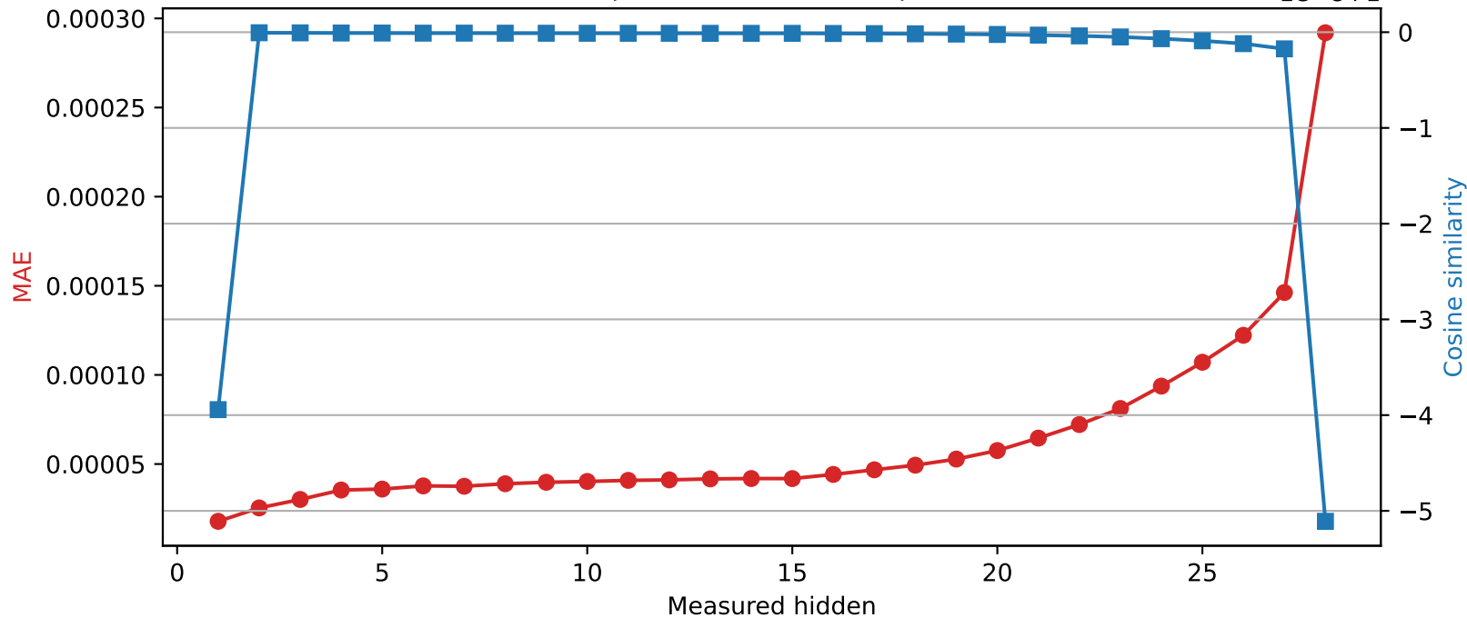
Llama-3.2-3B | Quantized layer 0 | float32 → int16
