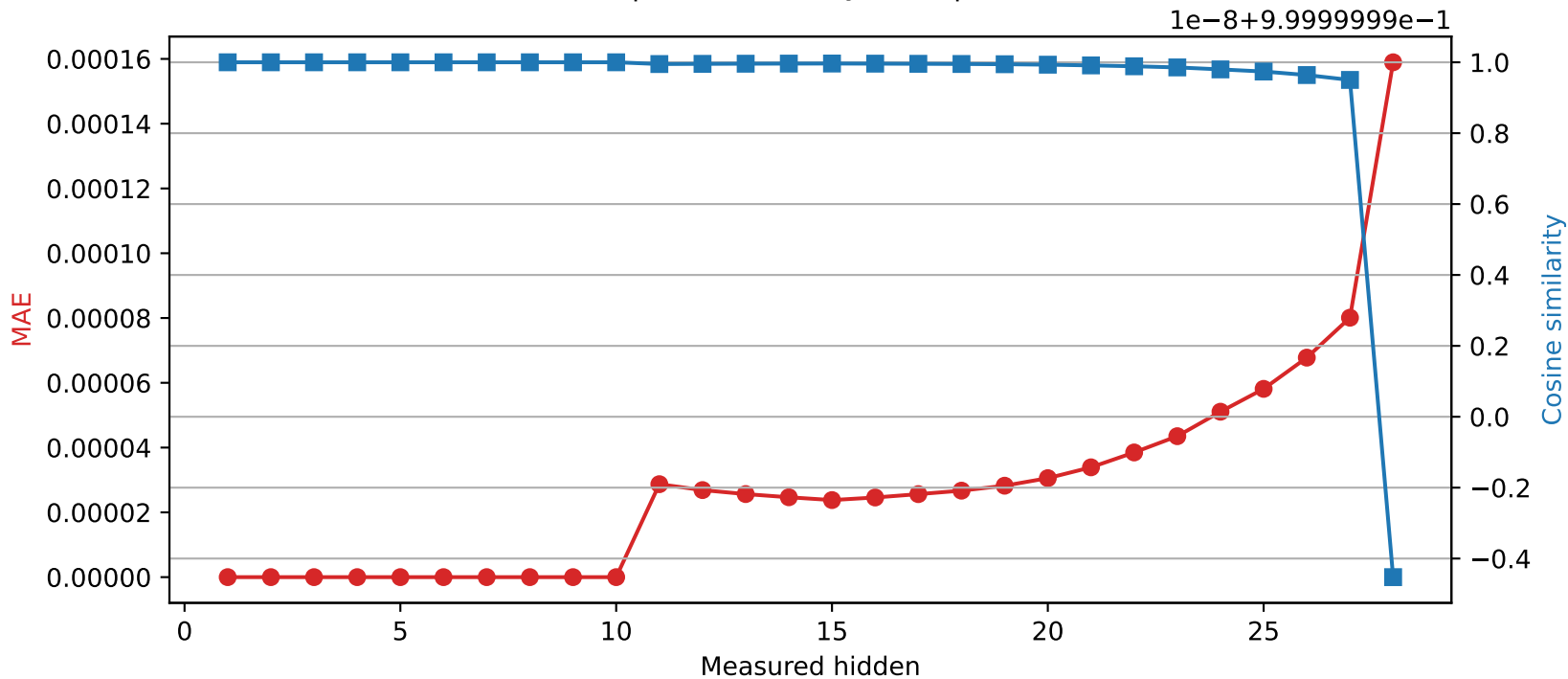
Llama-3.2-3B | Quantized layer 10 | float32 → int16
