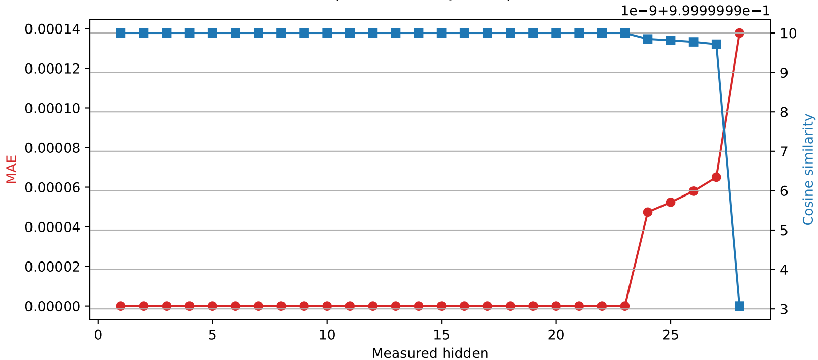
Llama-3.2-3B | Quantized layer 23 | float32 → int16
