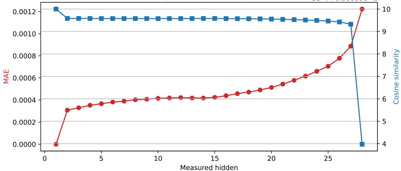
Llama-3.2-3B | Quantized layer 1 | float32 \rightarrow int16 1e-7+9.99999e-1
