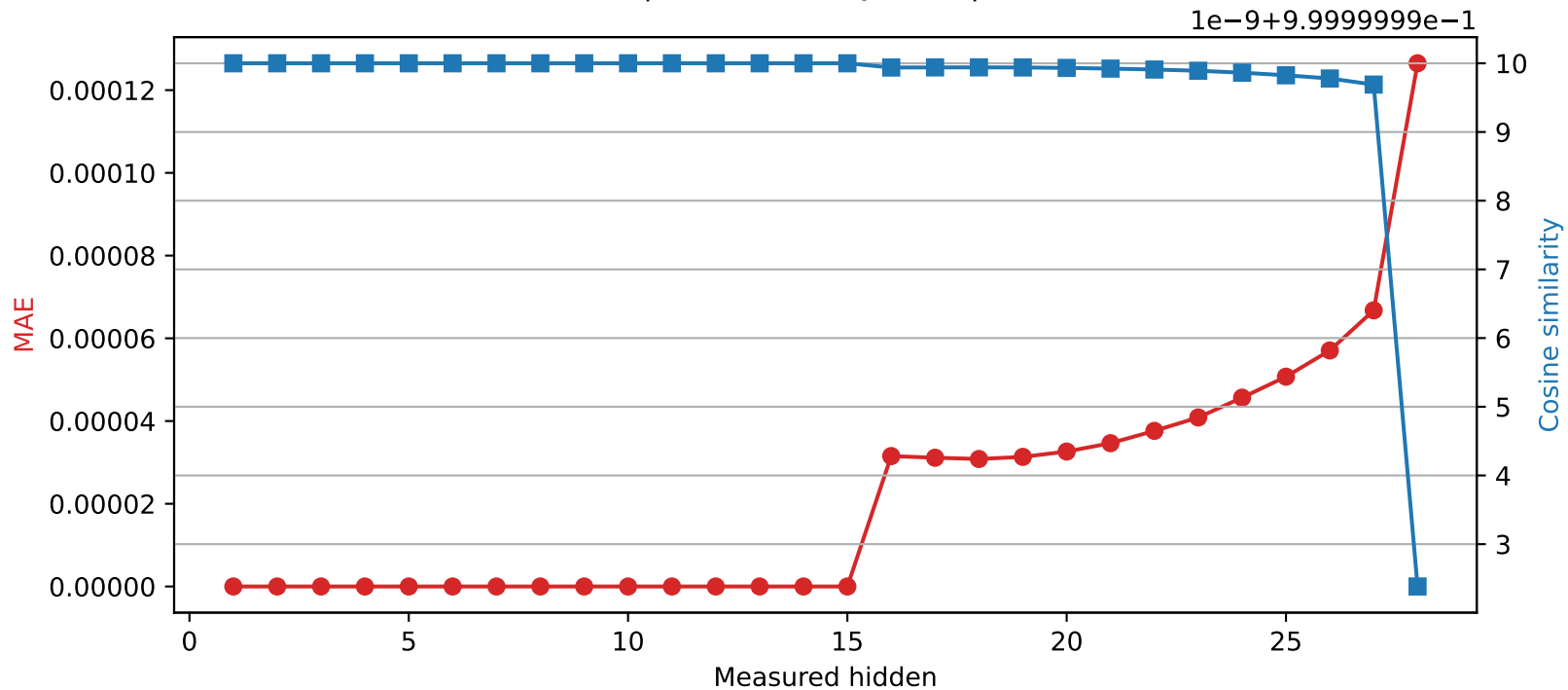
Llama-3.2-3B | Quantized layer 15 | float32 → int16
