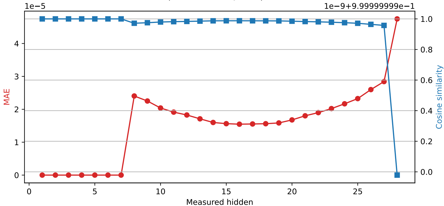
Llama-3.2-3B | Quantized layer 7 | float32 → int16
