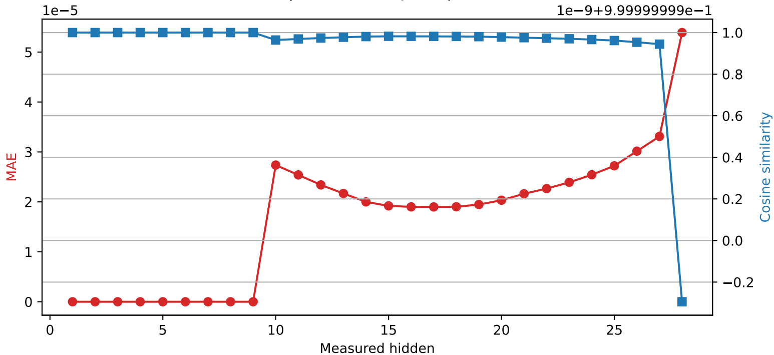
Llama-3.2-3B | Quantized layer 9 | float32 → int16
