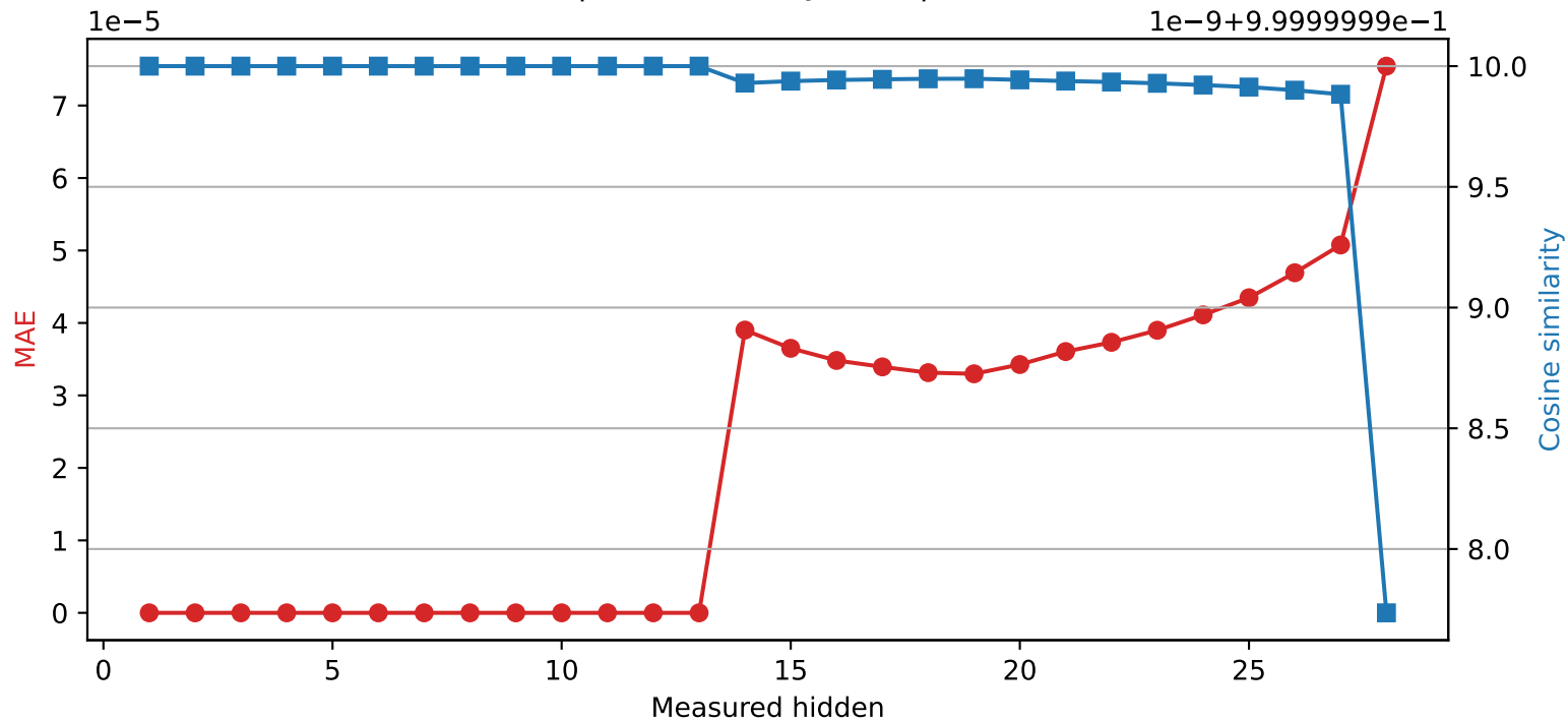
Llama-3.2-3B | Quantized layer 13 | float32 → int16
