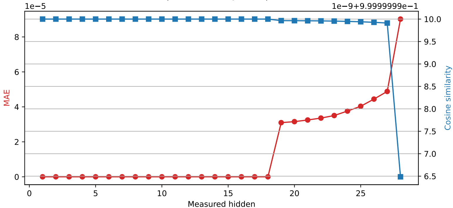
Llama-3.2-3B | Quantized layer 18 | float64 → int16
