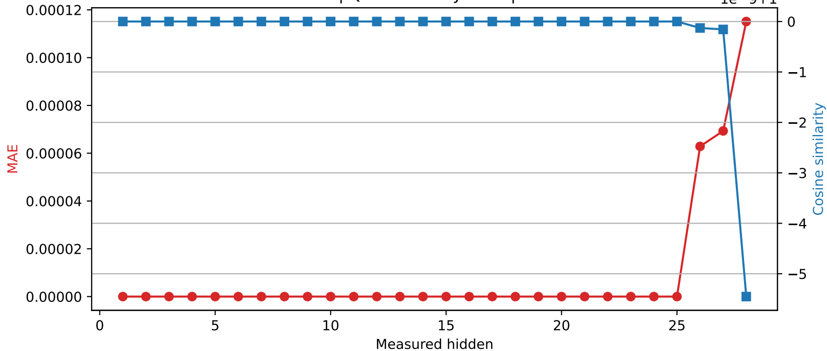
Llama-3.2-3B | Quantized layer 25 | float64 → int16
