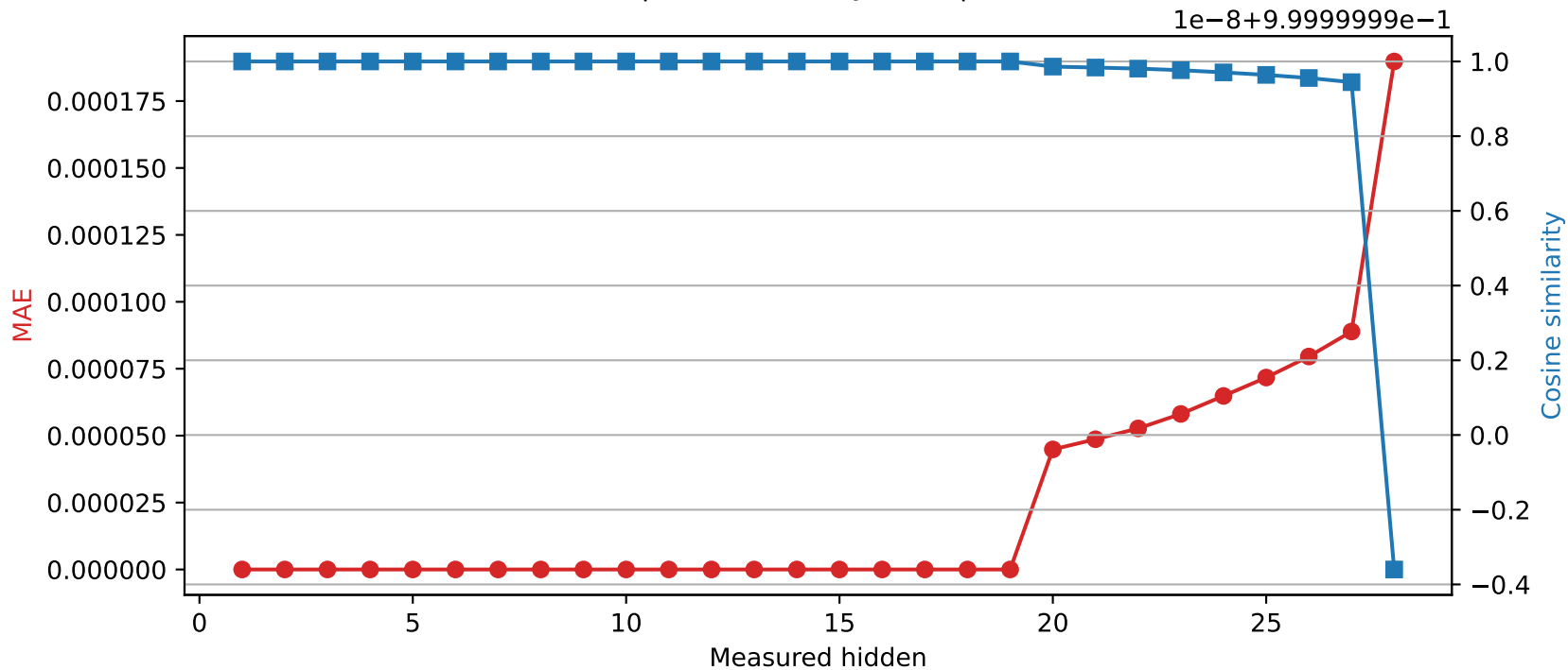
Llama-3.2-3B | Quantized layer 19 | float64 → int16
