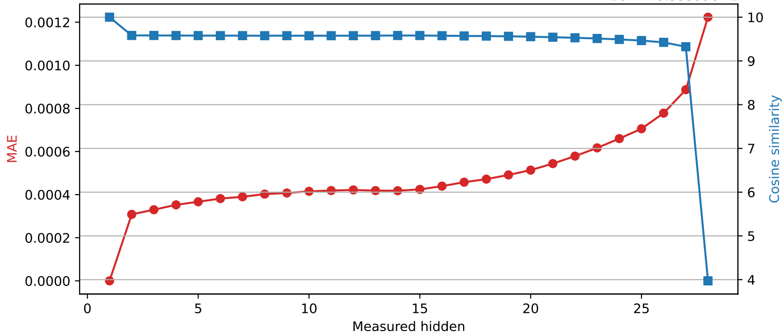
Llama-3.2-3B | Quantized layer 1 | float64 \rightarrow int16 1e-7+9.99999e-1
