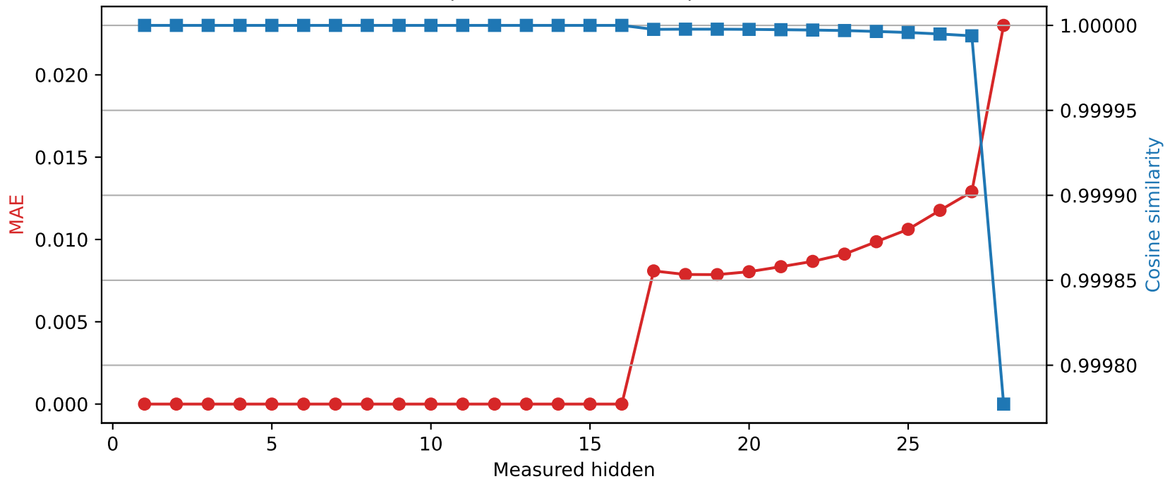
Llama-3.2-3B | Quantized layer 16 | float16 → int8
