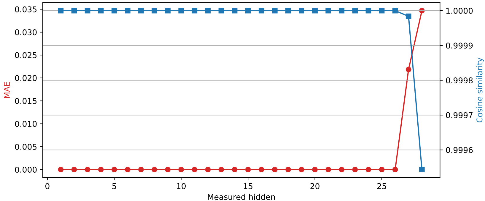
Llama-3.2-3B | Quantized layer 26 | float16 \rightarrow int8
