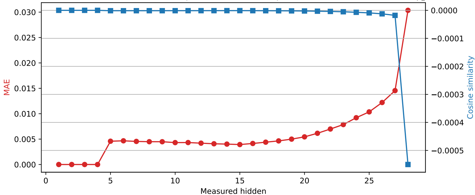
Llama-3.2-3B | Quantized layer 4 | float16 \rightarrow int8
