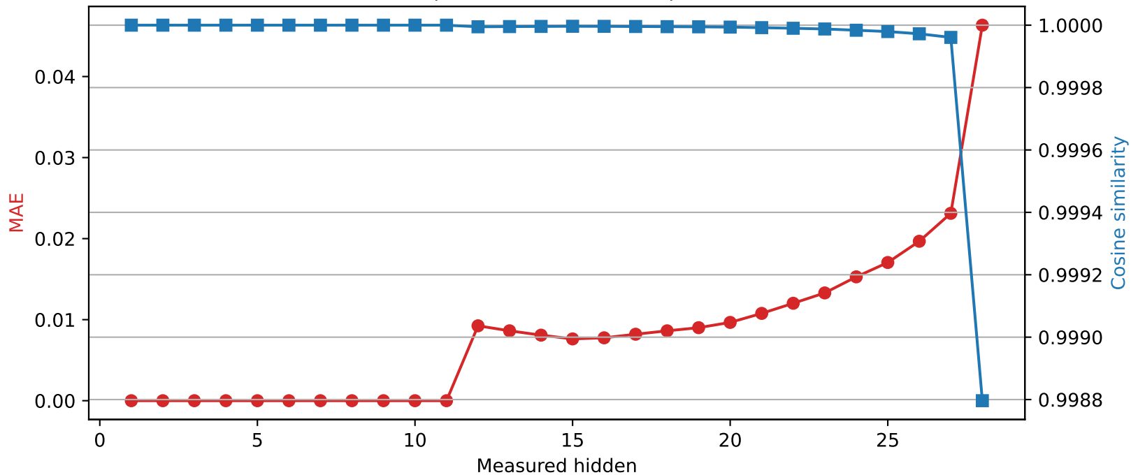
Llama-3.2-3B | Quantized layer 11 | float16 → int8
