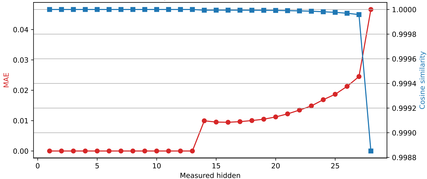
Llama-3.2-3B | Quantized layer 13 | float16 \rightarrow int8
