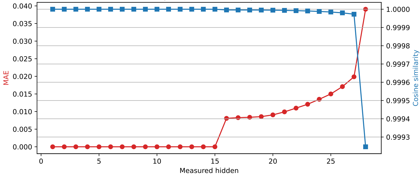
Llama-3.2-3B | Quantized layer 15 | float16 \rightarrow int8
