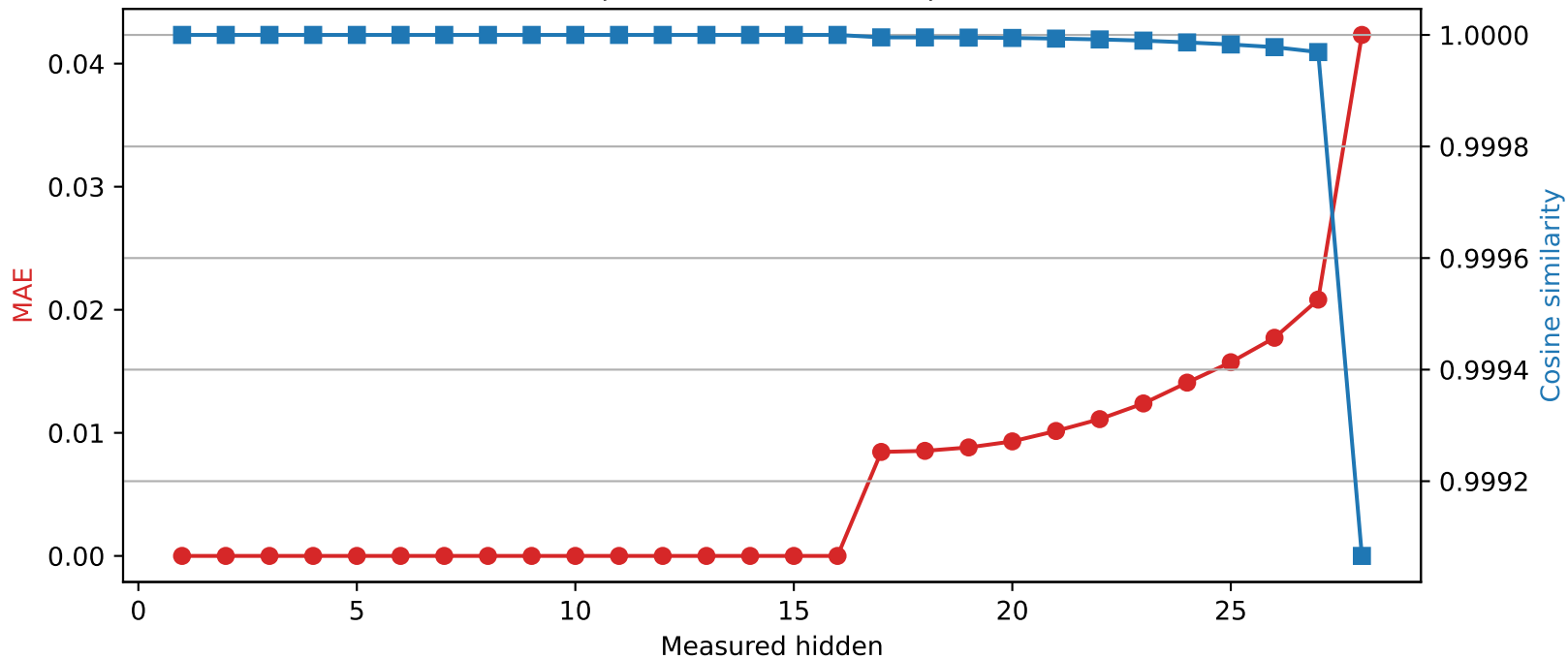
Llama-3.2-3B | Quantized layer 16 | float16 \rightarrow int8
