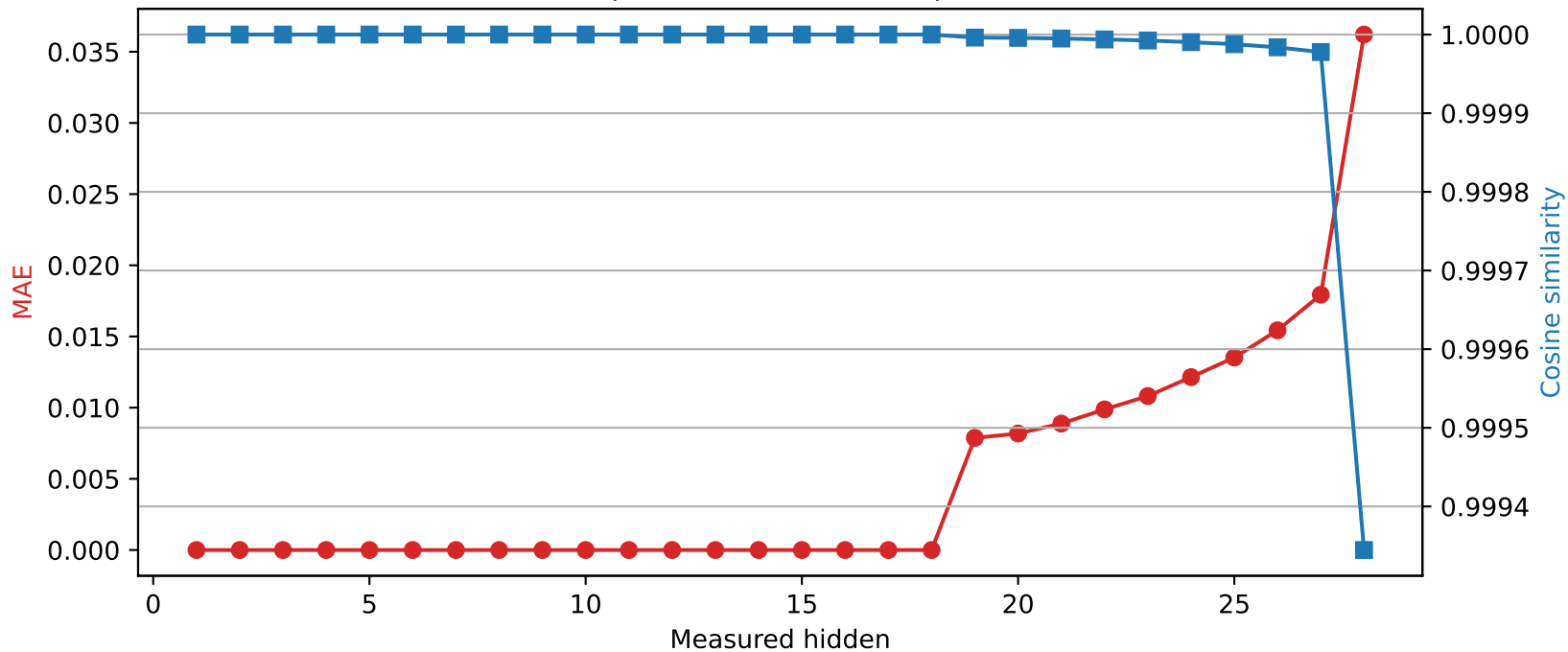
Llama-3.2-3B | Quantized layer 18 | float16 → int8
