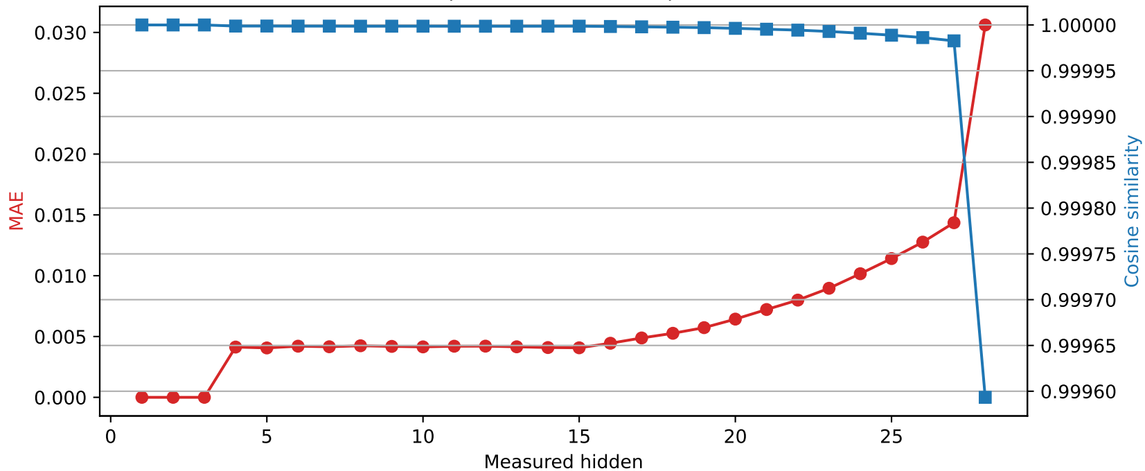
Llama-3.2-3B | Quantized layer 3 | float16 → int8
