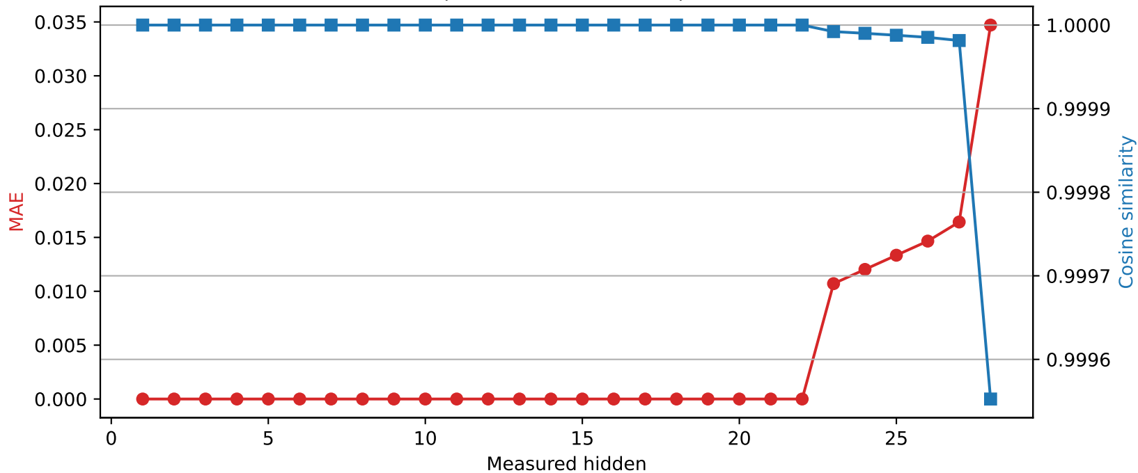
Llama-3.2-3B | Quantized layer 22 | float16 \rightarrow int8
