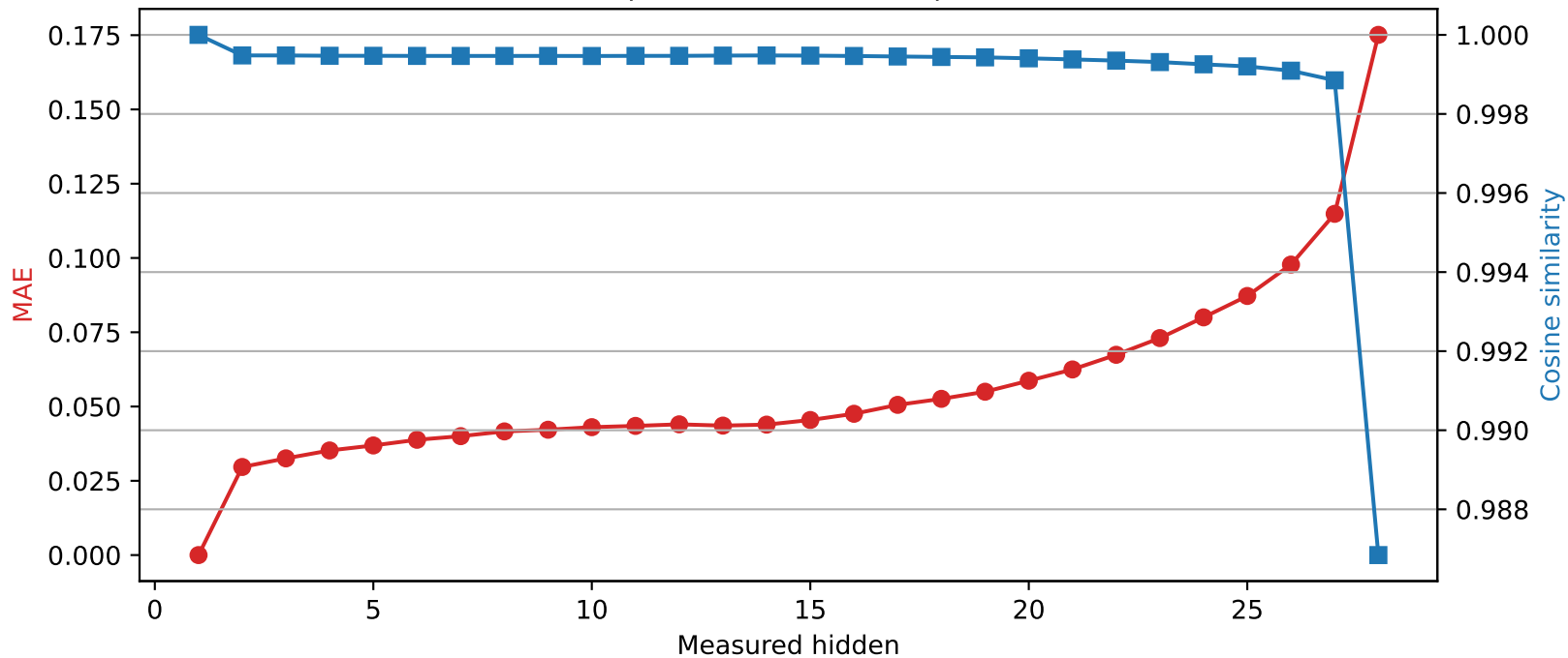
Llama-3.2-3B | Quantized layer 1 | float16 \rightarrow int8
