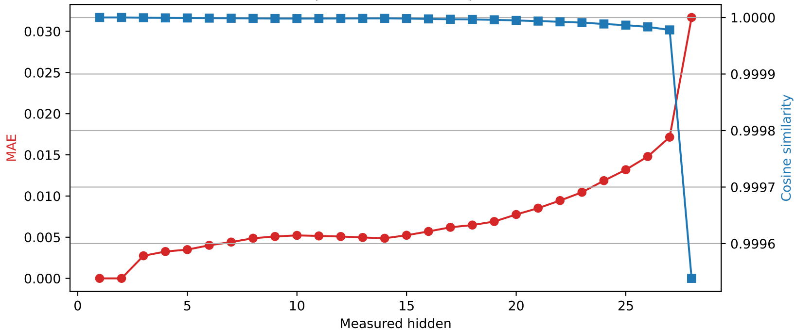
Llama-3.2-3B | Quantized layer 2 | float16 \rightarrow int8
