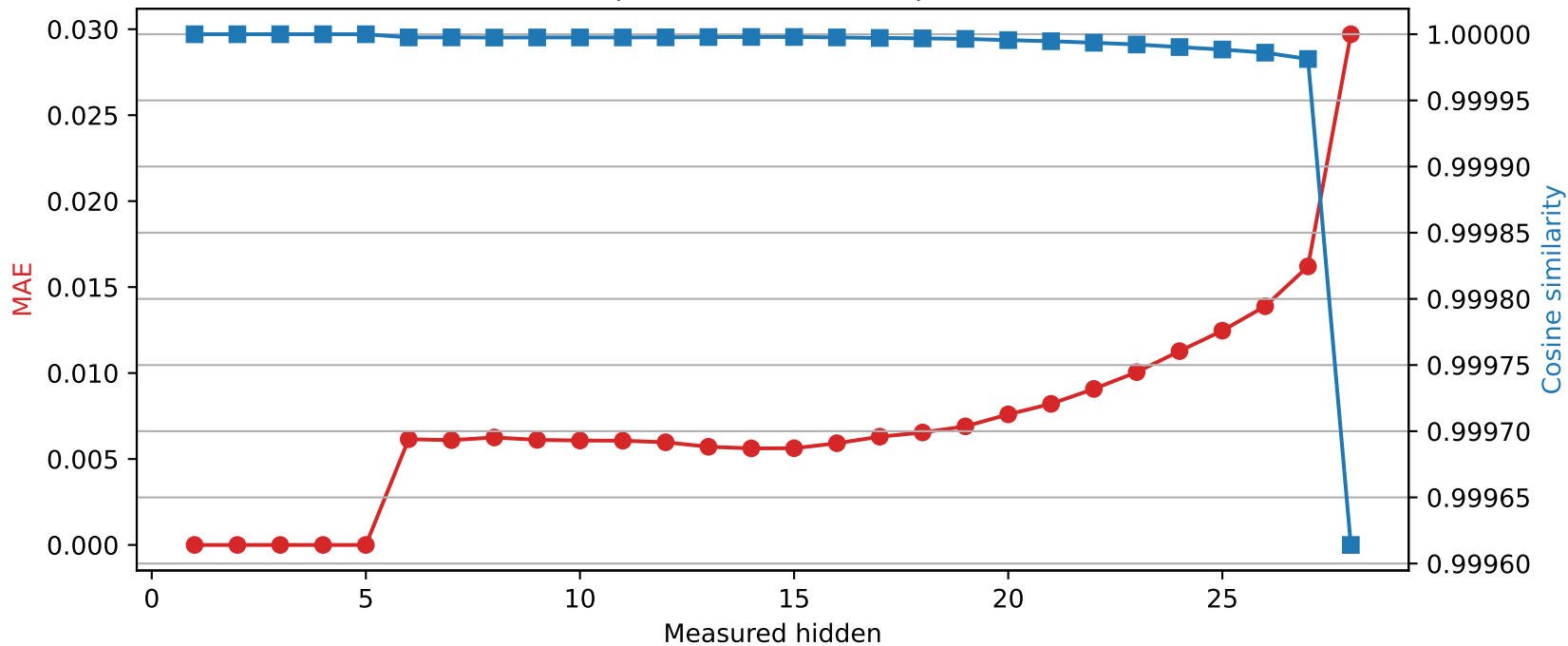
Llama-3.2-3B | Quantized layer 5 | float16 → int8
