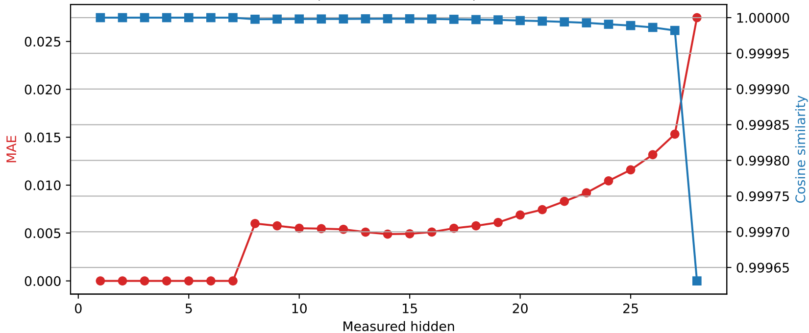
Llama-3.2-3B | Quantized layer 7 | float16 → int8
