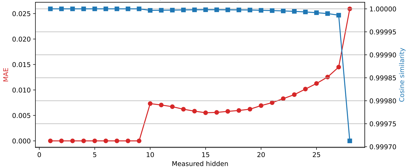
Llama-3.2-3B | Quantized layer 9 | float16 → int8
