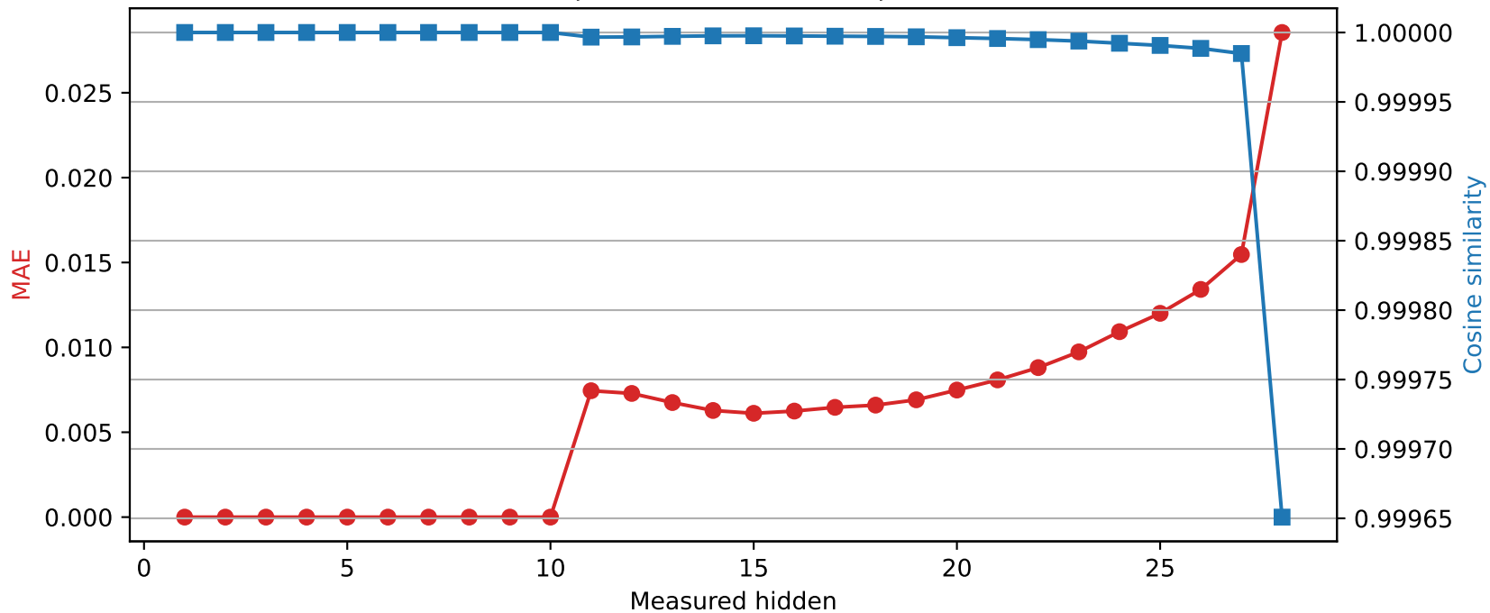
Llama-3.2-3B | Quantized layer 10 | float16 \rightarrow int8
