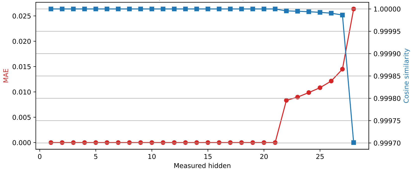
Llama-3.2-3B | Quantized layer 21 | float16 → int8
