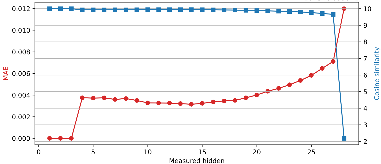
Llama-3.2-3B | Quantized layer 3 | float16 → int8
