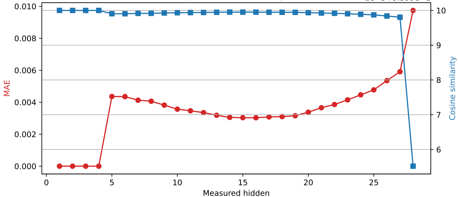
Llama-3.2-3B | Quantized layer 4 | float16 → int8
