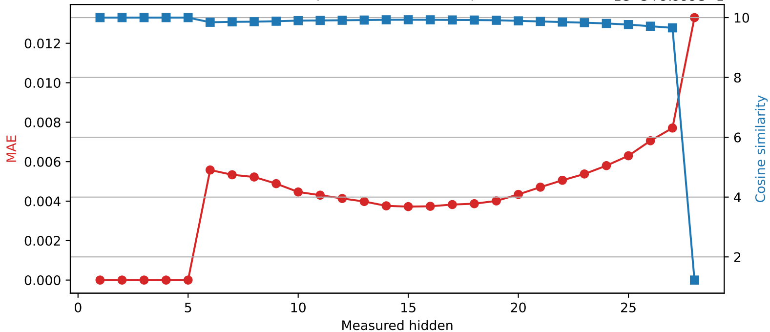
Llama-3.2-3B | Quantized layer 5 | float16 → int8
