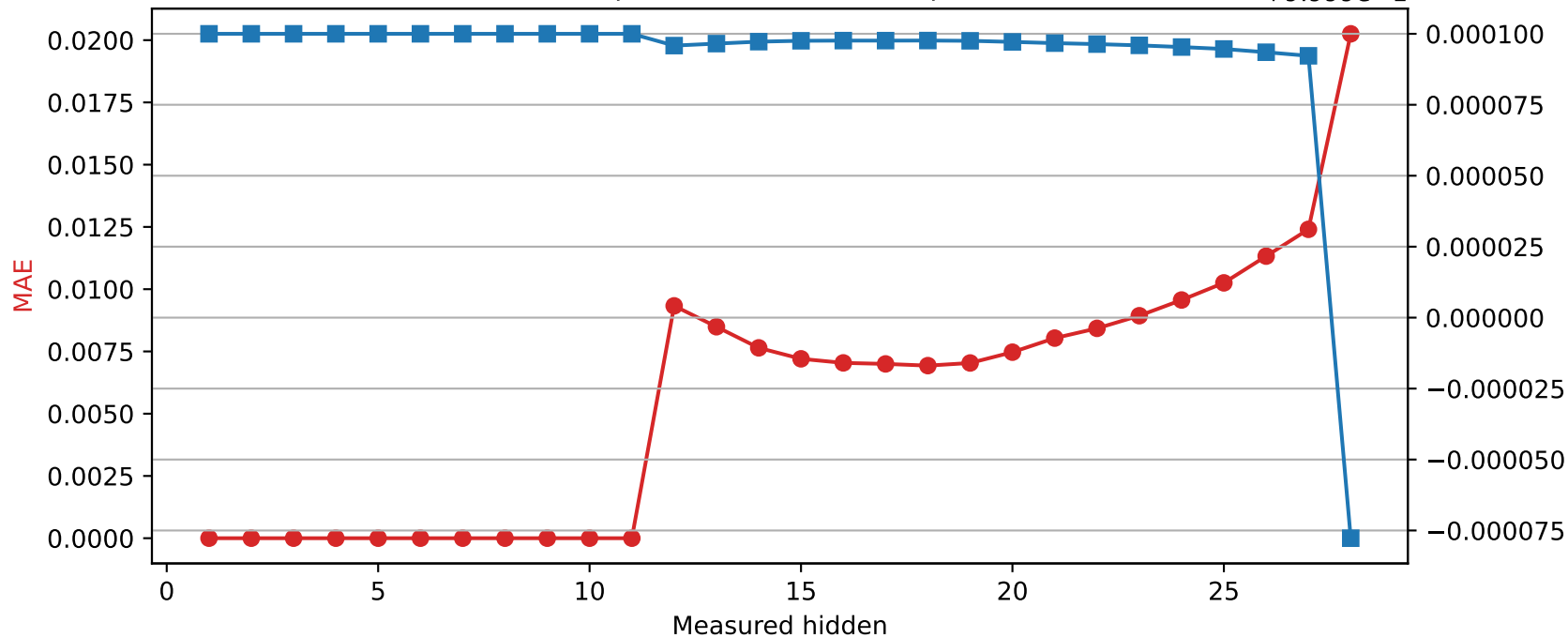
Llama-3.2-3B | Quantized layer 11 | float16 \rightarrow int8
